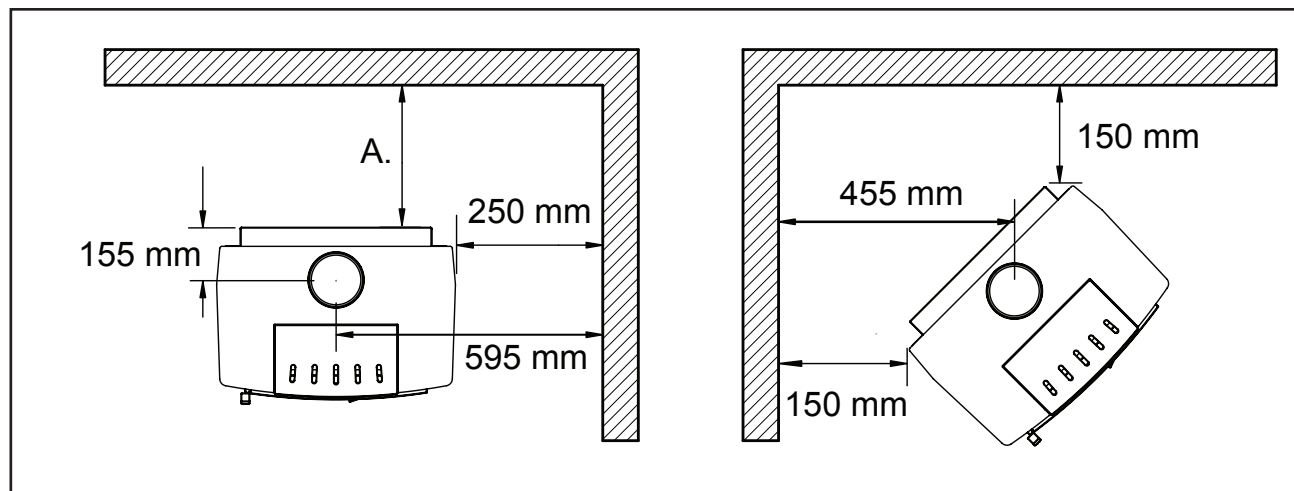
Figure 4. Neo 1.6 Clearances
