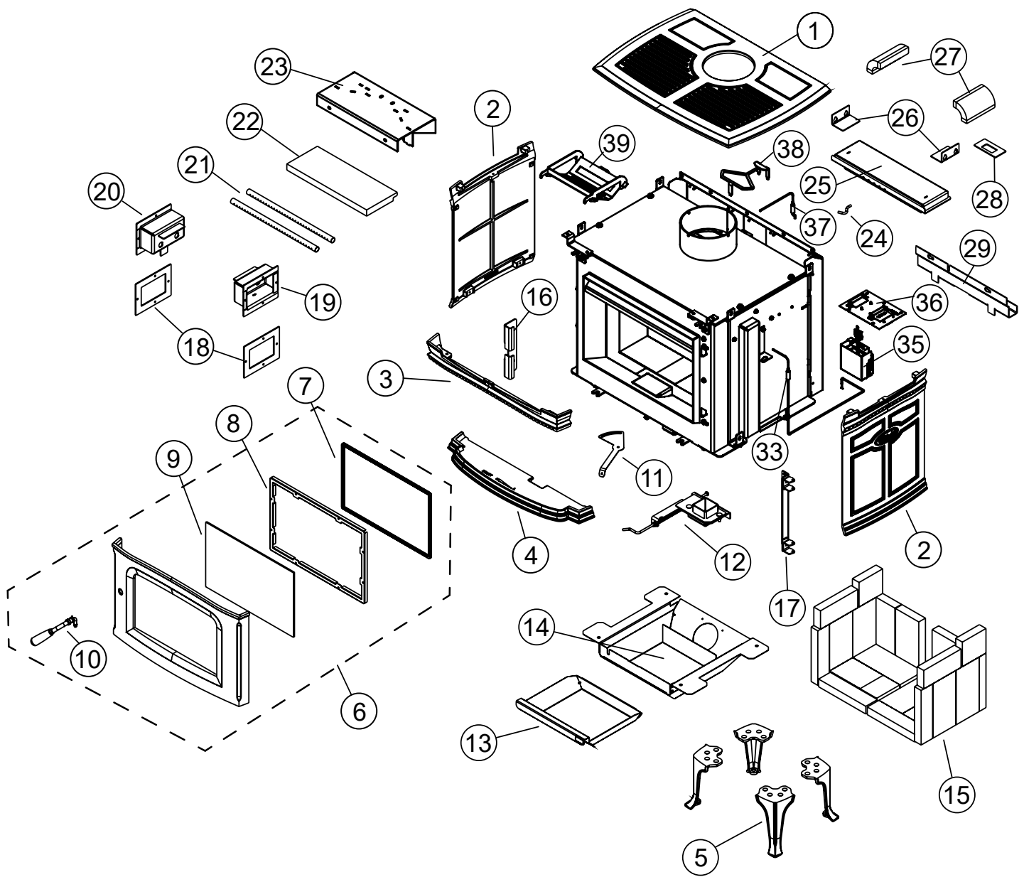
Figure 28. ALT4 LE2 AS Replacement parts.
