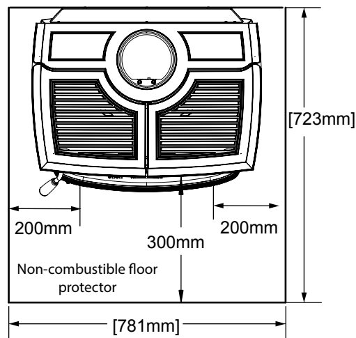
Figure 12. ALT4 LE2 AS Hearth pad.
