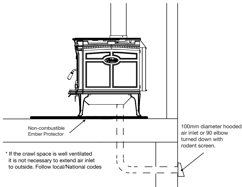
Figure 27. ALT AS Fresh Air.
