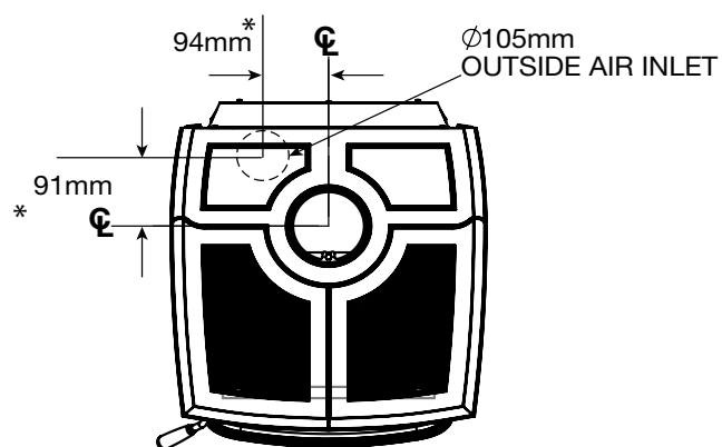
Figure 2. OUTSIDE AIR DIMS metric.
