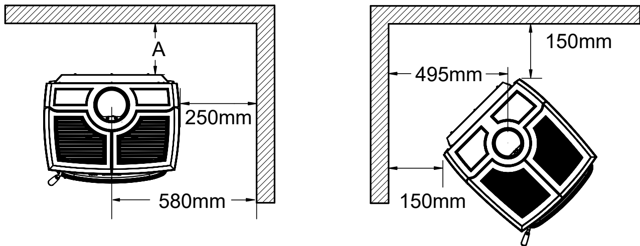
Figure 11. ALT4 LE2 AS Clearances.
